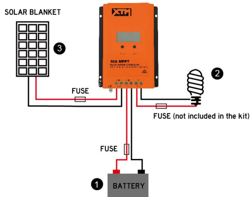
Wiring Diagram
