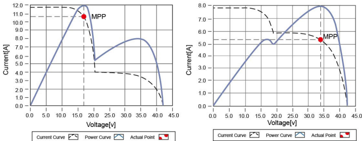
Figure 1-3 Mutil-MPP Curve
