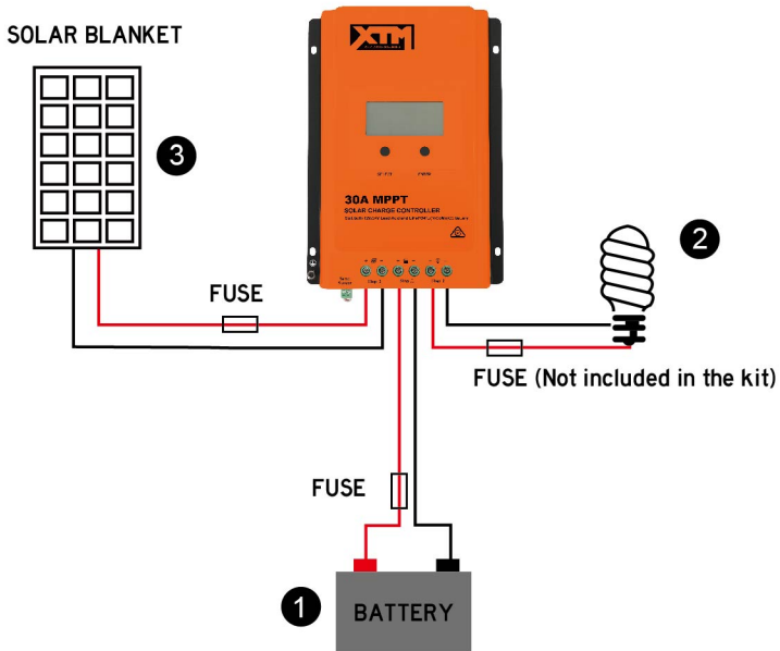
Wiring Diagram
